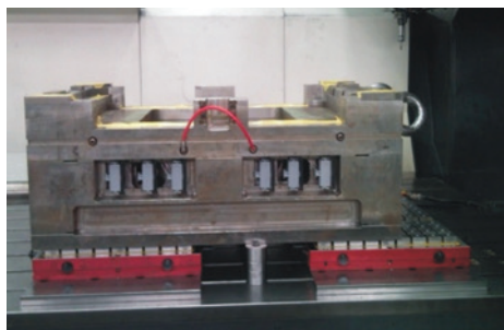
Machining injection mold application
