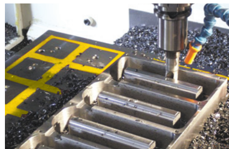
Machining mold cavities
