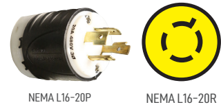
NEMA L16-20P NEMA L16-20R NEMA L16-20P plug comes installed on the power cord. Requires a NEMA L16-20R receptacle.
